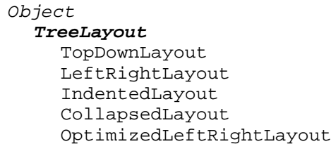
Figure 14. The TreeLayout Hierarchy.
